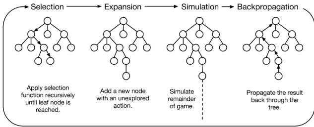
Figure 1: Outline of Monte-Carlo Tree Search
